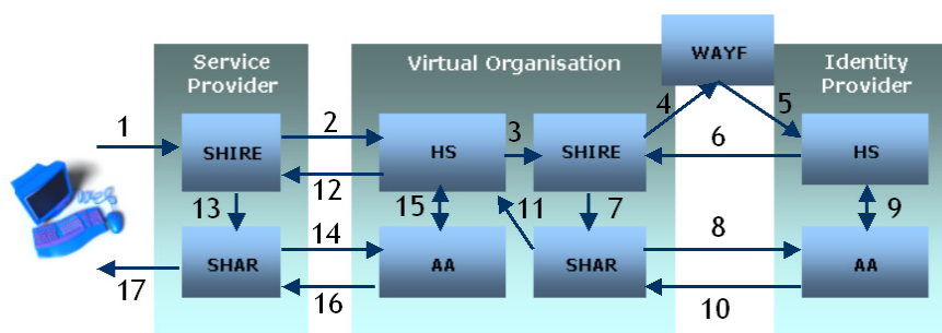
Figure 1: the Virtual Organization Service Provider
